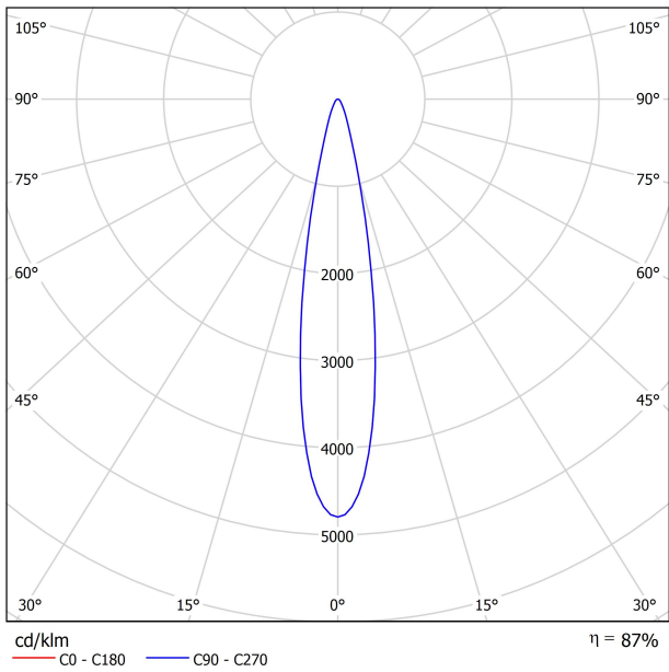
POLAR DIAGRAM
